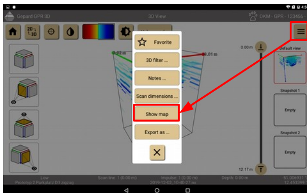
Figure 7.27: Create a map file - Alternative 1
