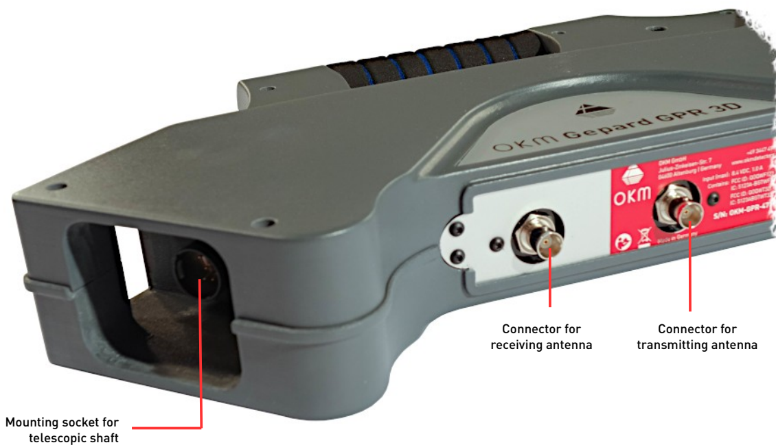
Figure 4.2: Connector panel of the control unit
